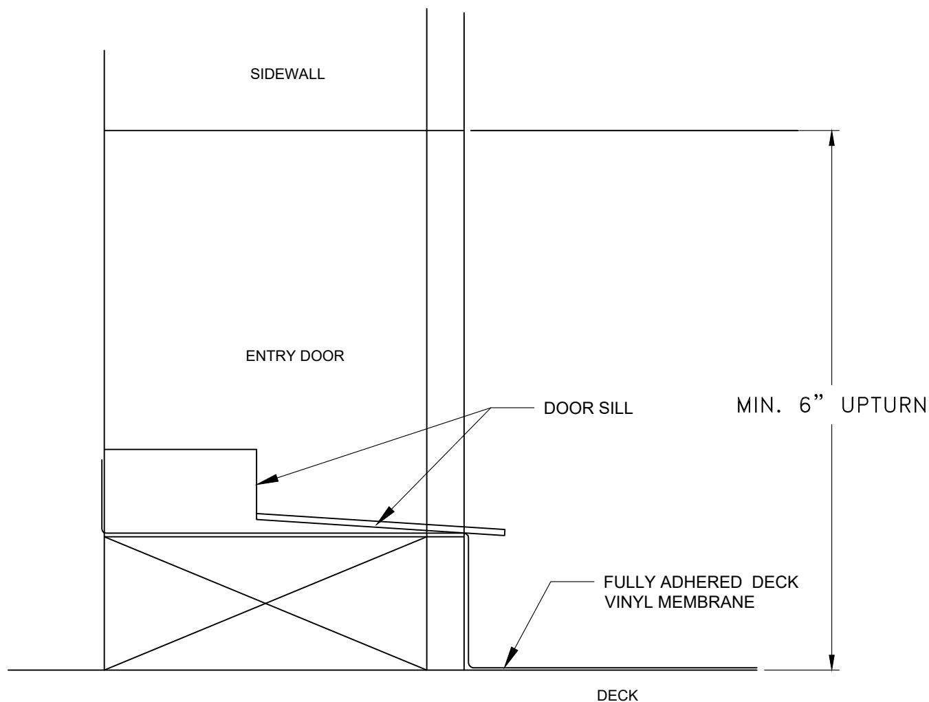
SECTION VIEW
