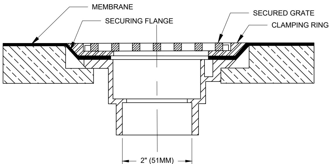
SECTION VIEW
